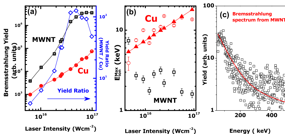
FIG. 2. (Color online) (a) Bremsstrahlung yield recorded from MWNT (black) and Cu (red) samples with laser intensity. The ratio of the bremsstrahlung yield (blue) from both the samples is plotted in the same graph with a different y-axis (right). MWNT sample produced two orders of magnitude larger x-ray flux. (b) shows the maximum ion energies recorded from MWNT (black) and Cu (red) under identical experimental conditions. The solid line in this figure shows that Cu ion energy follows (\lambda^2)^{0.4} scaling. Note that MWNTs do not follow this scaling. (c) Bremsstrahlung spectrum from MWNT. The solid line shows a hot electron component at 36 keV. The low energy component is not shown here. The data for the polished Cu have been reported earlier by us. (See the references, Rajeev et al. , 2002 and 2003.)
