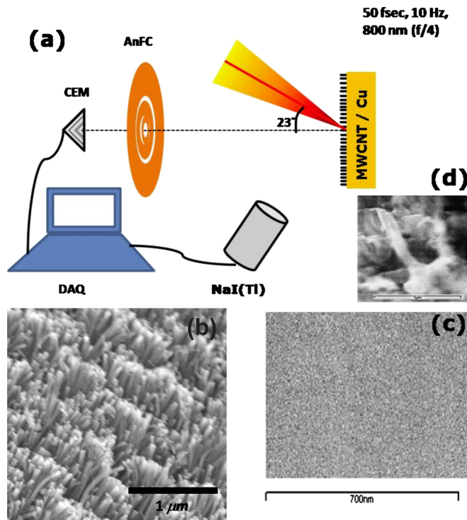
FIG. 1. (Color online) Schematic experimental arrangement is shown in (a). The ion energies along the target normal direction are measured using CEM, and AnFCs are employed to estimate the angular divergence of the ion emission. SEM image (top view) of the MWCNT and polished copper (Cu) are shown in (b) and (c), respectively. A SEM image of an individual MWCNT is shown in (d).
