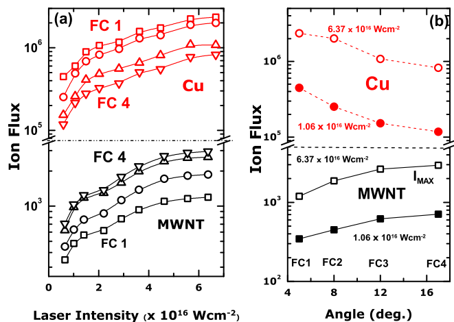
FIG. 3. (Color online) The ion flux recorded by the AnFCs for MWNT (black) and Cu (red) are shown in (a). Three orders of magnitude reduction in on debris from MWNT sample are evident. Angle resolved ion flux distribution is plotted in (b). With increasing laser intensity, the ion flux for Cu (red) peaks around the target normal direction whereas, in contradiction, in case of MWNT, the flux become more divergent in nature.
